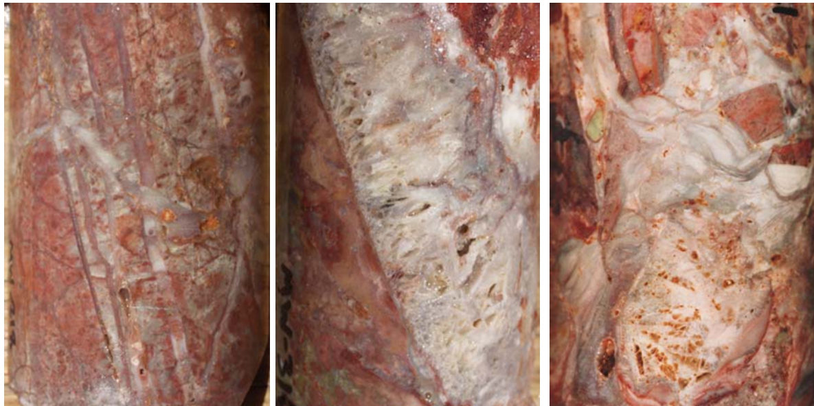
Figure 7-8: Core Photos of Tonopah Vein Structures
